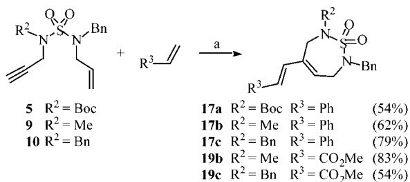
Scheme 4. Reagents: (a) 2a (6 mol%), \text{CH}_2\text{Cl}_2 , microwave irradiation (100 °C)
